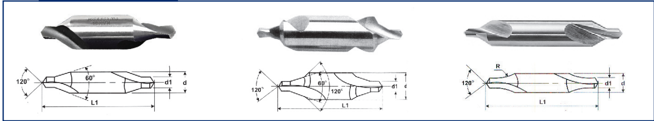
HSS CENTRE DRILL TYPE-A IS : 6708 - 1977 DIN : 333
